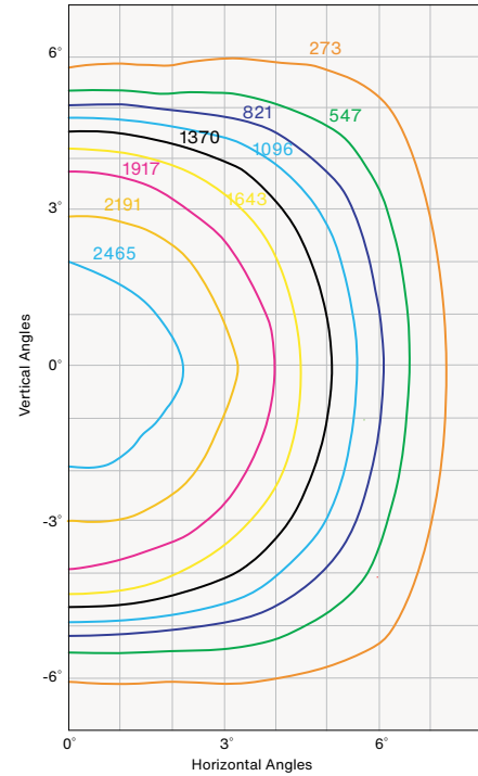
Isocandela Curves
